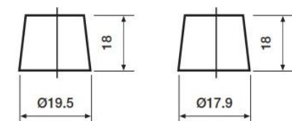
Positive Terminal
