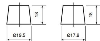
Positive Terminal
